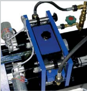
Grease flow control valve Solid construction, 20 mm Steel plates.
